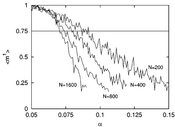
FIG. 2. Retrieval of a pattern in a neural network with depressing synapses at T=0 . The figure shows the average overlap of the final state of the network with the starting pattern as a function of the loading parameter \alpha and for different network sizes. Here, we have considered, for illustrative purposes, the particular situation for \gamma=1 . The lines represent the average overlap obtained in N_r = 150 retrieval experiments for each value of \alpha . The value \langle m^1 \rangle = 0.75 is used as a criterion to define \alpha_c .
